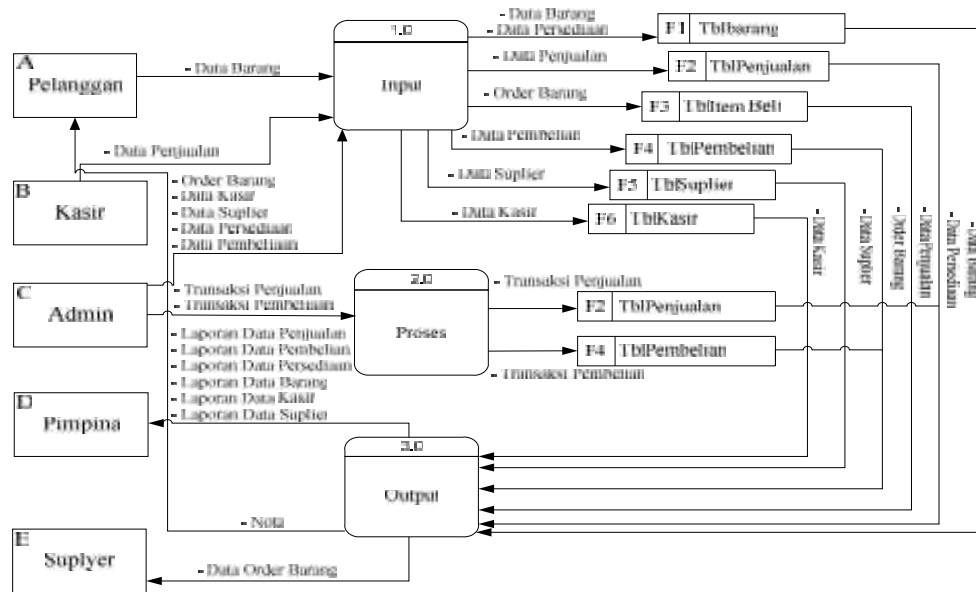
Gambar 4. Diagram Arus Data Level 0
