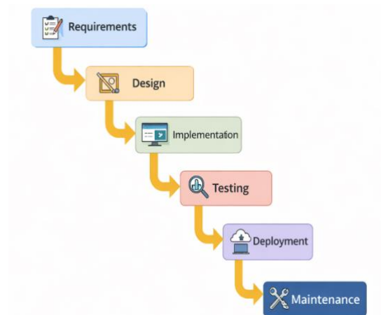
Gambar 2. Model Waterfall
