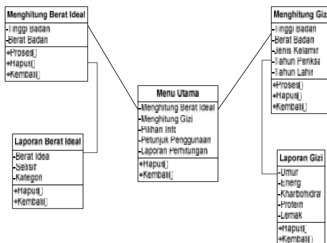
Gambar 3. Class Diagram
